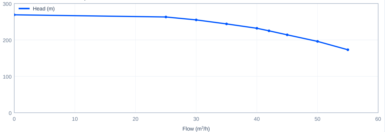
Head versus flow - CDM42-11, 50 Hz
