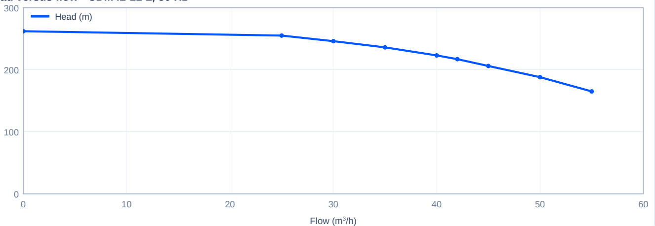
Head versus flow - CDM42-11-2, 50 Hz
