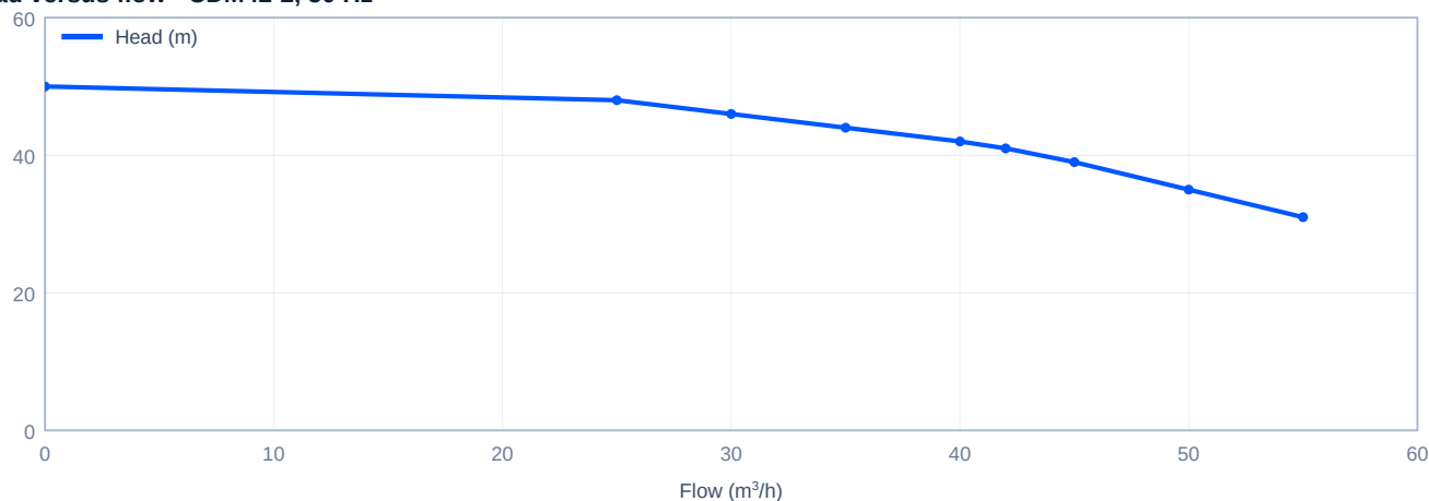
Head versus flow - CDM42-2, 50 Hz
