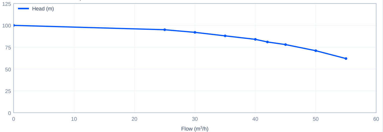
Head versus flow - CDM42-4, 50 Hz
