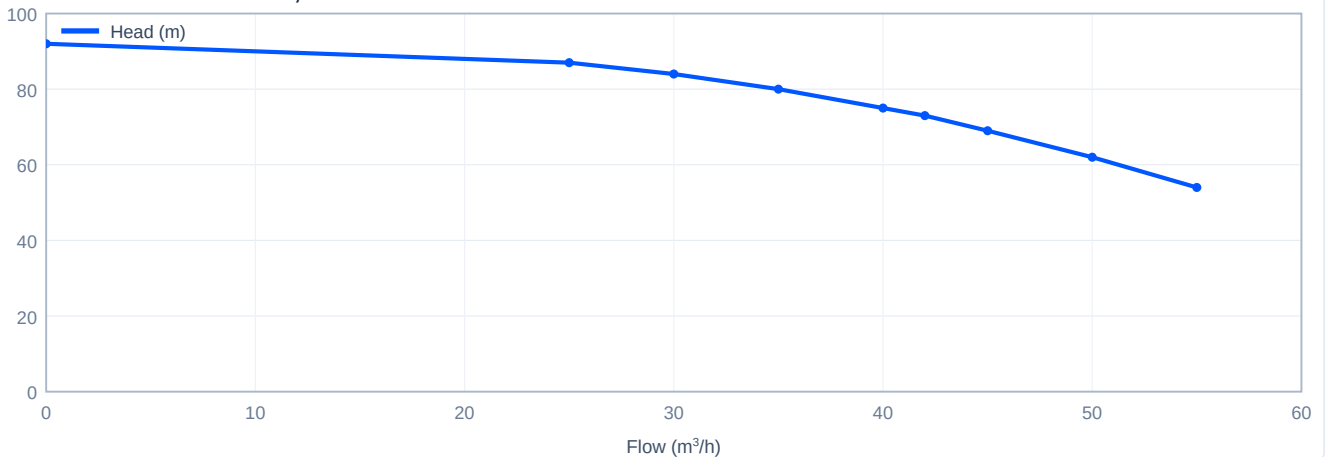
Head versus flow - CDM42-4-2, 50 Hz
