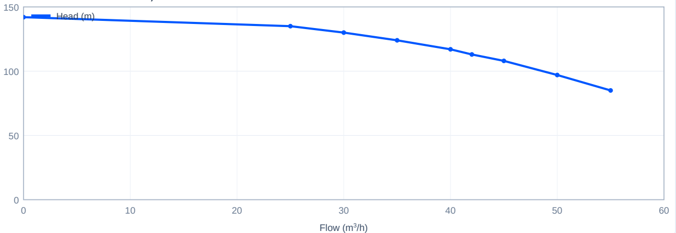
Head versus flow - CDM42-6-2, 50 Hz
