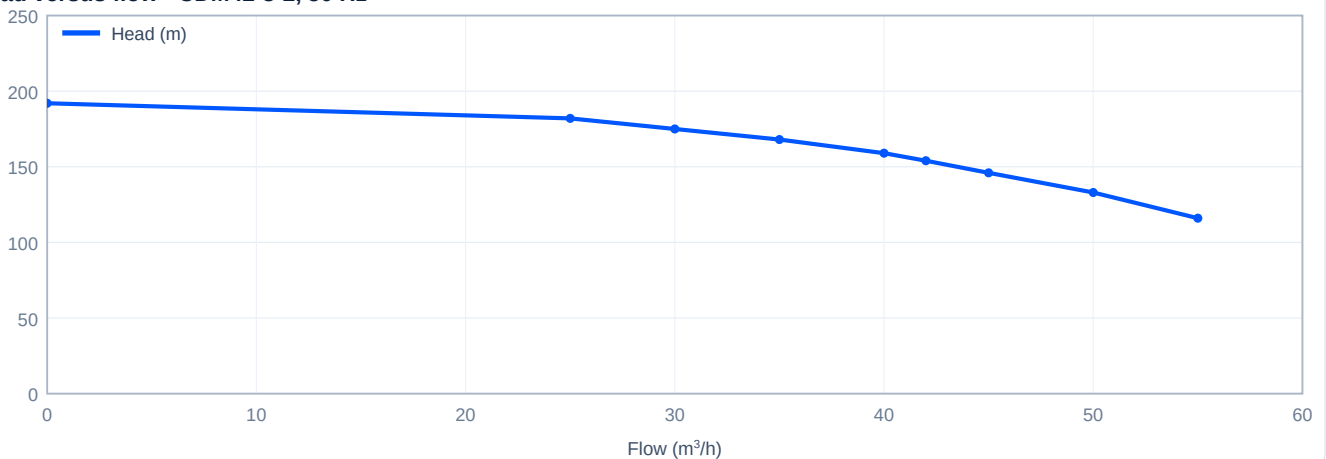
Head versus flow - CDM42-8-2, 50 Hz
