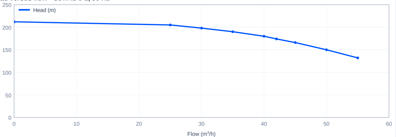
Head versus flow - CDM42-9-2, 50 Hz
