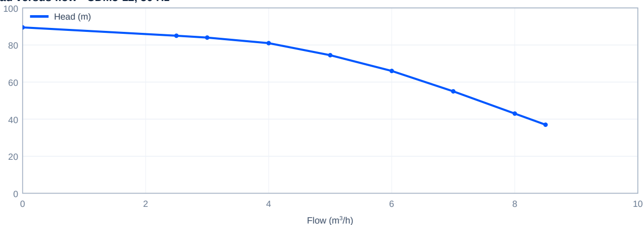
Head versus flow - CDM5-12, 50 Hz
