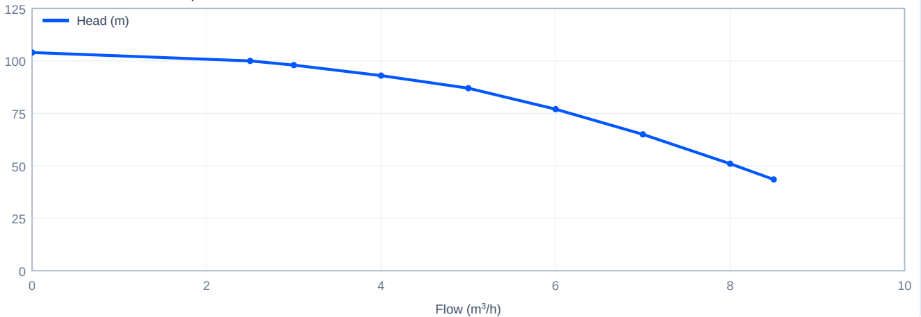
Head versus flow - CDM5-14, 50 Hz
