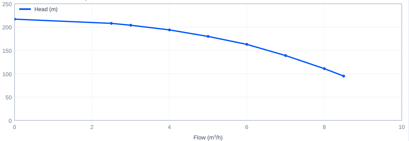
Head versus flow - CDM5-29, 50 Hz
