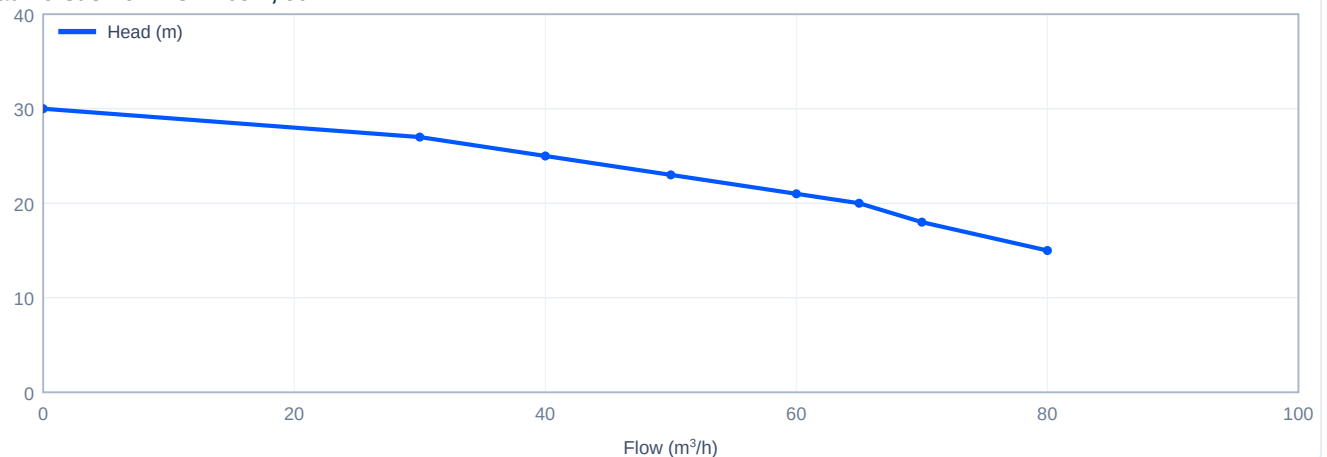
Head versus flow - CDM65-1, 50 Hz
