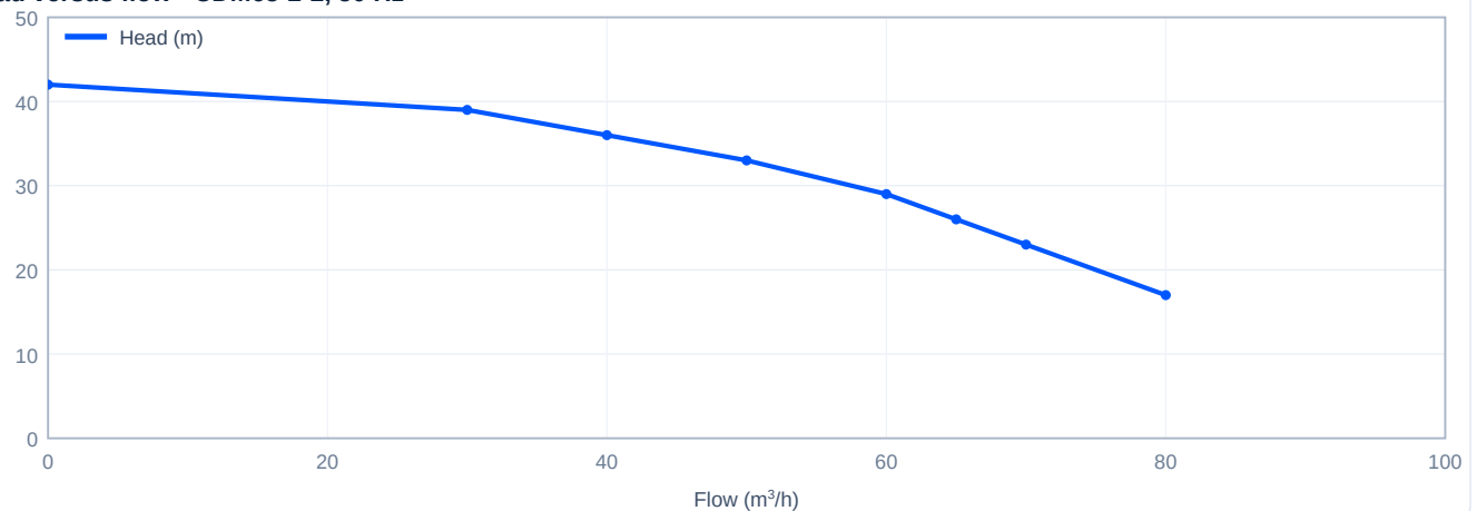
Head versus flow - CDM65-2-2, 50 Hz
