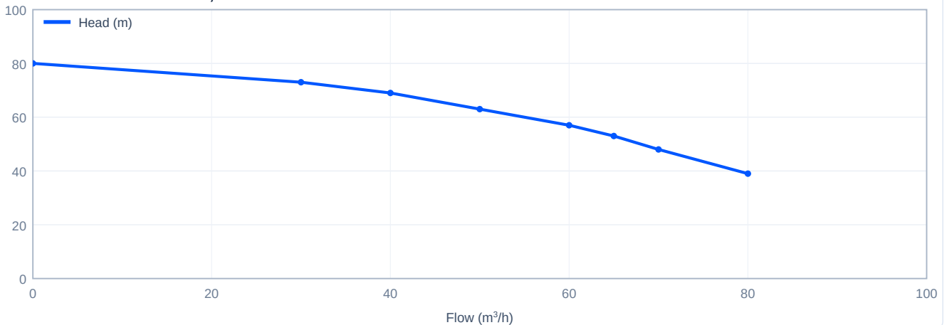
Head versus flow - CDM65-3-1, 50 Hz
