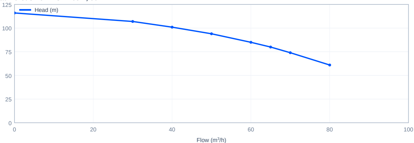
Head versus flow - CDM65-4, 50 Hz
