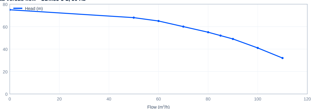
Head versus flow - CDM85-3-2, 50 Hz
