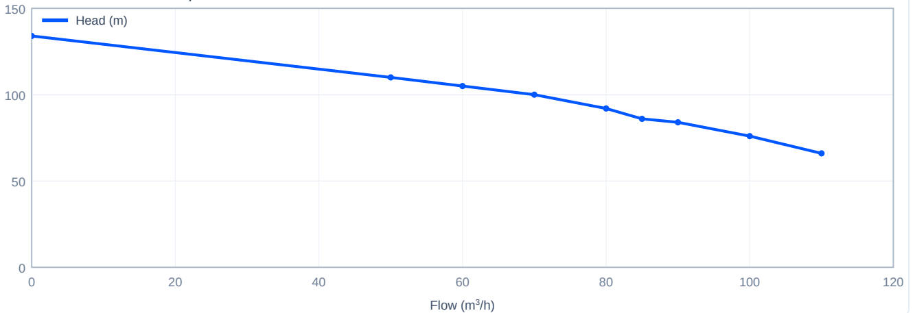
Head versus flow - CDM85-4, 50 Hz
