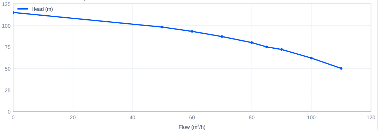
Head versus flow - CDM85-4-2, 50 Hz
