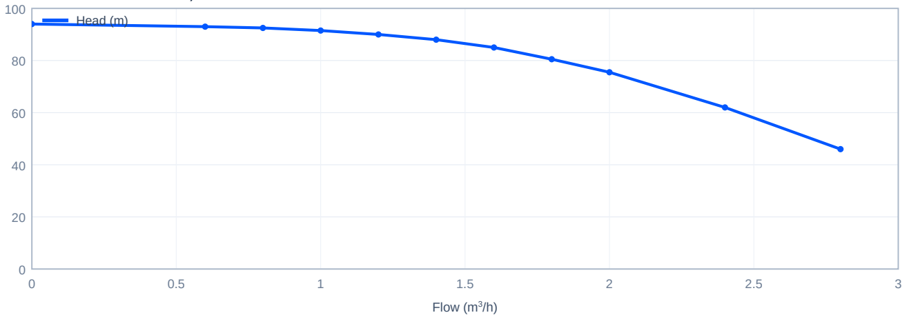
Head versus flow - CDM1-11, 60 Hz
