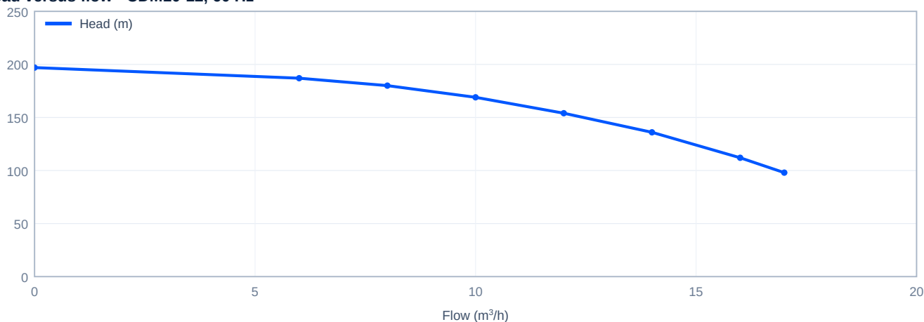
Head versus flow - CDM10-12, 60 Hz
