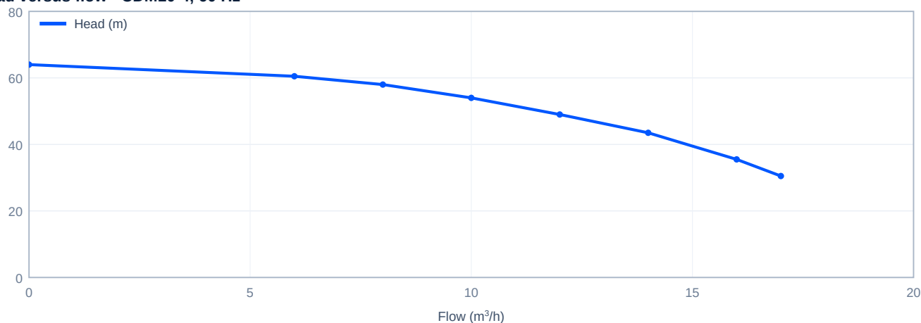
Head versus flow - CDM10-4, 60 Hz
