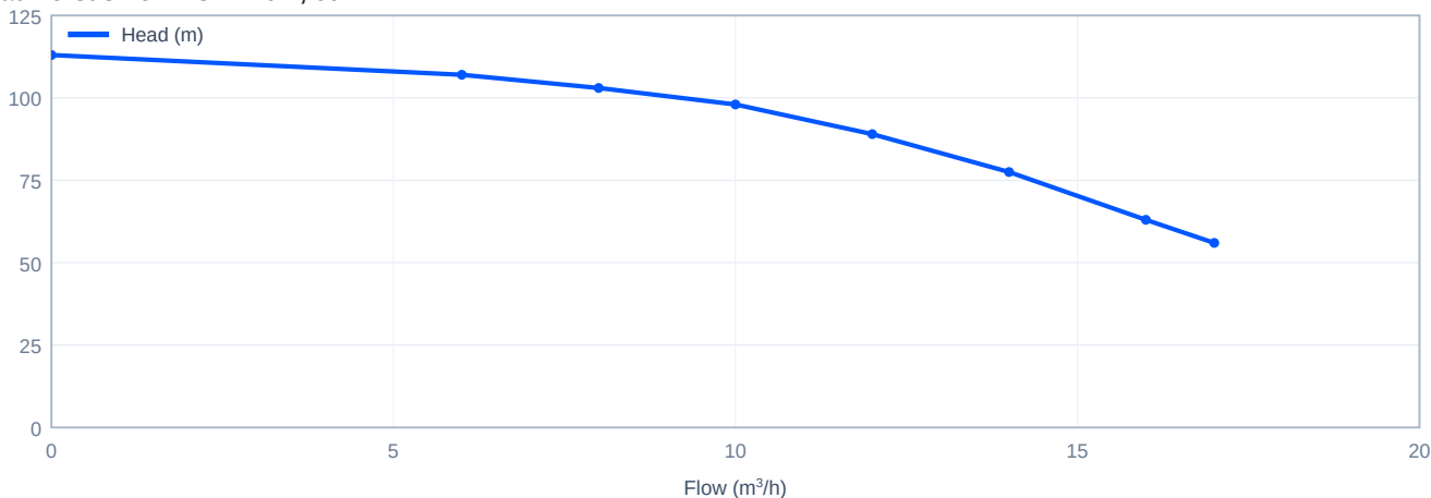
Head versus flow - CDM10-7, 60 Hz
