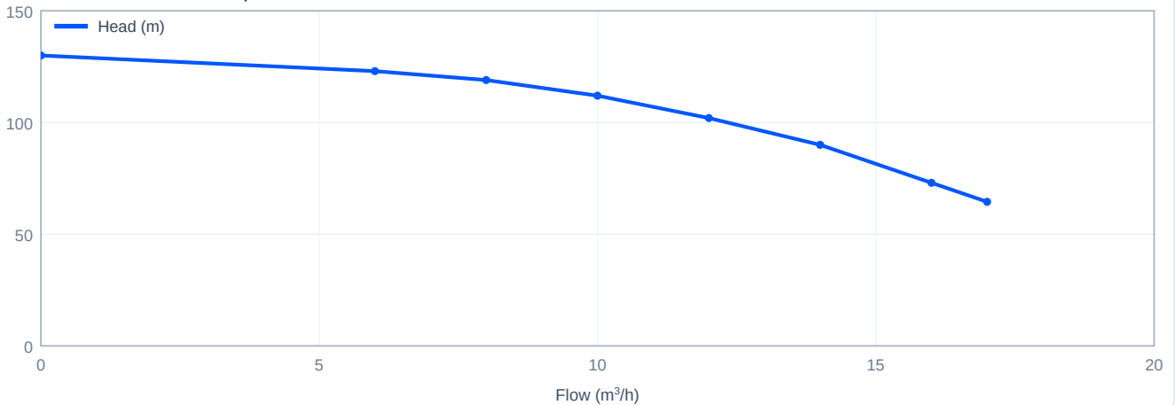
Head versus flow - CDM10-8, 60 Hz
