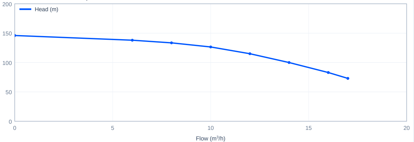
Head versus flow - CDM10-9, 60 Hz
