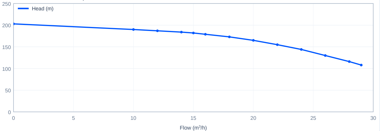
Head versus flow - CDM15-10, 60 Hz
