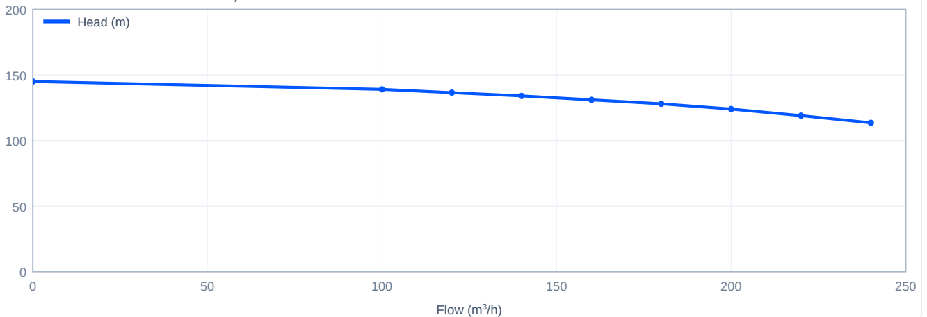
Head versus flow - CDM200-3-A-B, 60 Hz
