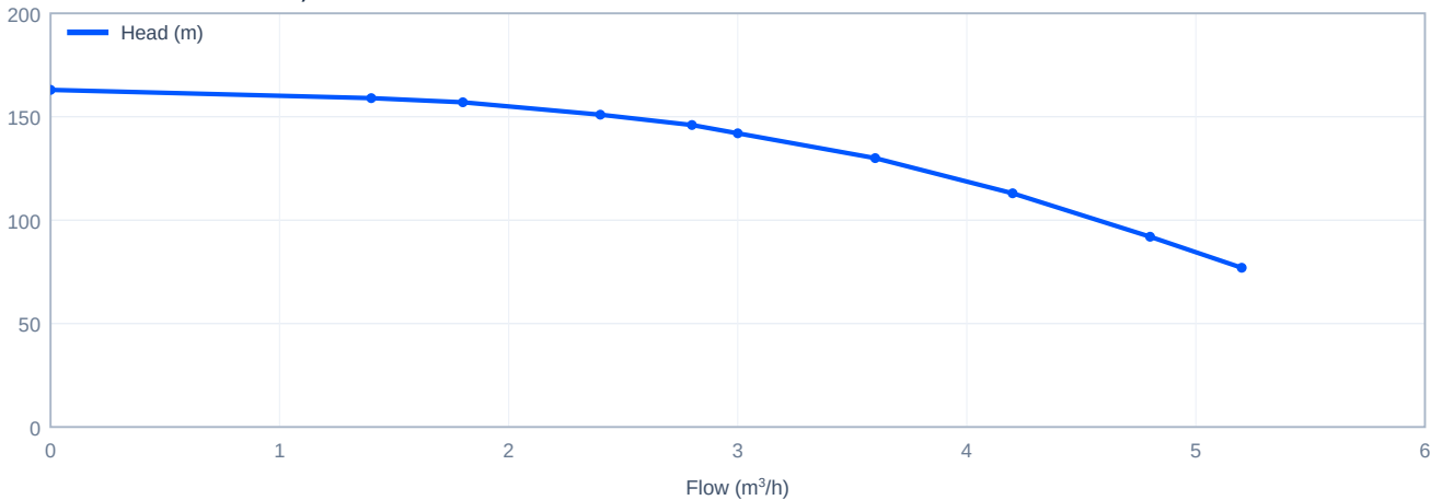
Head versus flow - CDM3-15, 60 Hz
