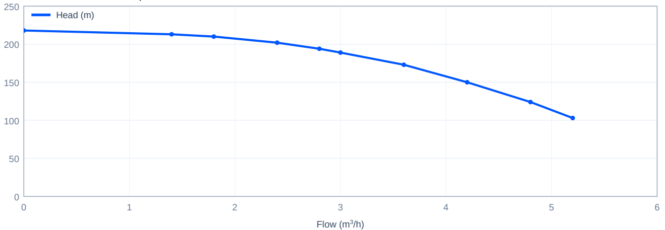
Head versus flow - CDM3-20, 60 Hz
