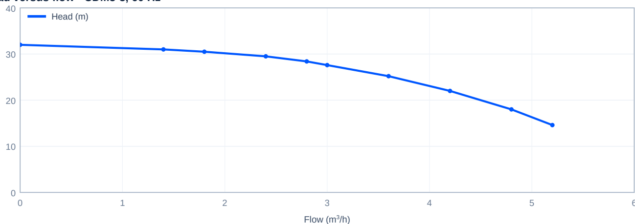
Head versus flow - CDM3-3, 60 Hz
