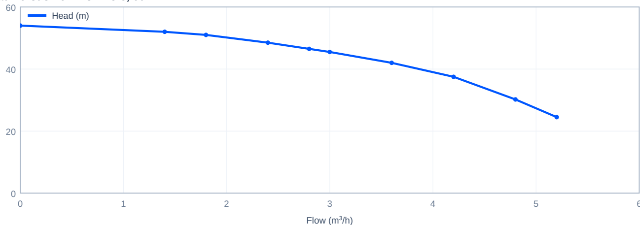
Head versus flow - CDM3-5, 60 Hz
