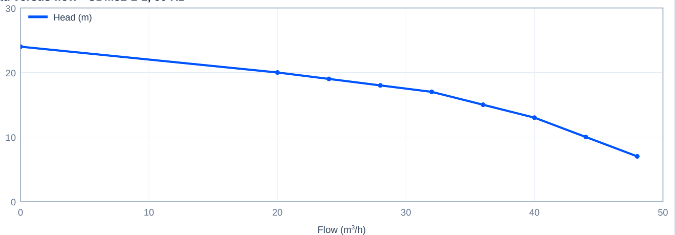
Head versus flow - CDM32-1-1, 60 Hz
