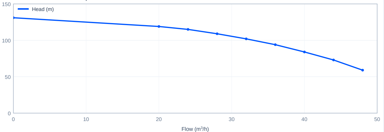
Head versus flow - CDM32-5-2, 60 Hz
