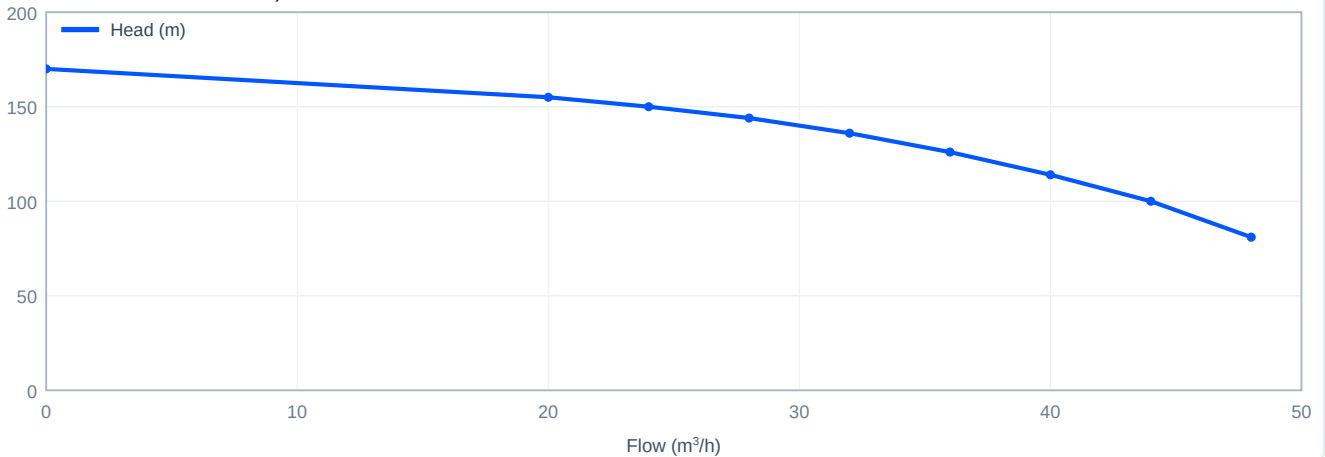
Head versus flow - CDM32-6, 60 Hz
