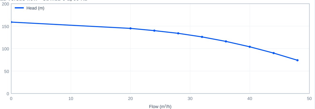
Head versus flow - CDM32-6-2, 60 Hz
