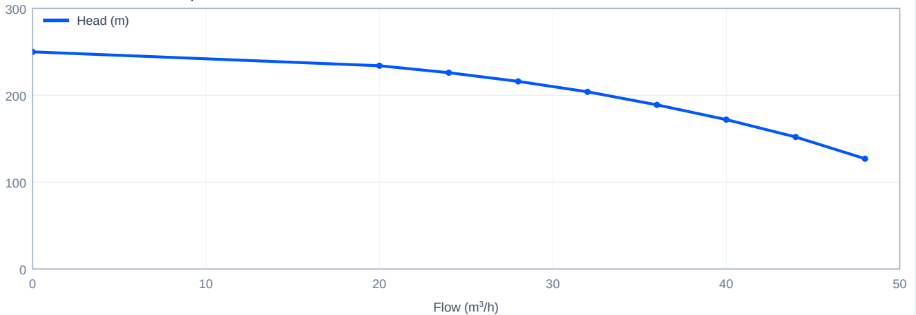
Head versus flow - CDM32-9, 60 Hz
