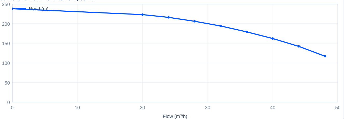
Head versus flow - CDM32-9-2, 60 Hz
