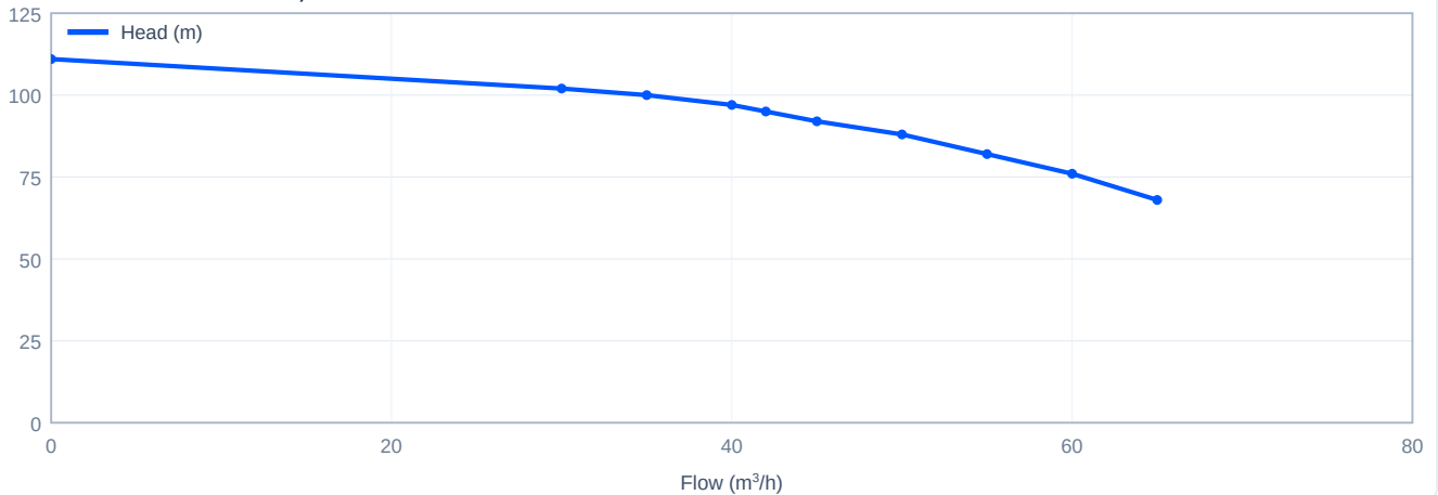
Head versus flow - CDM42-3, 60 Hz
