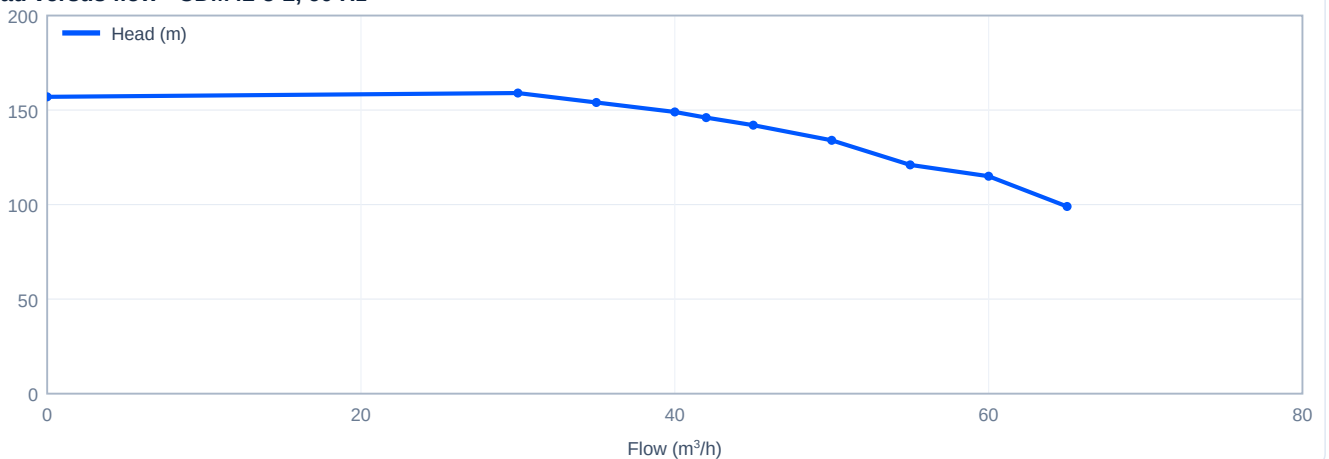
Head versus flow - CDM42-5-2, 60 Hz
