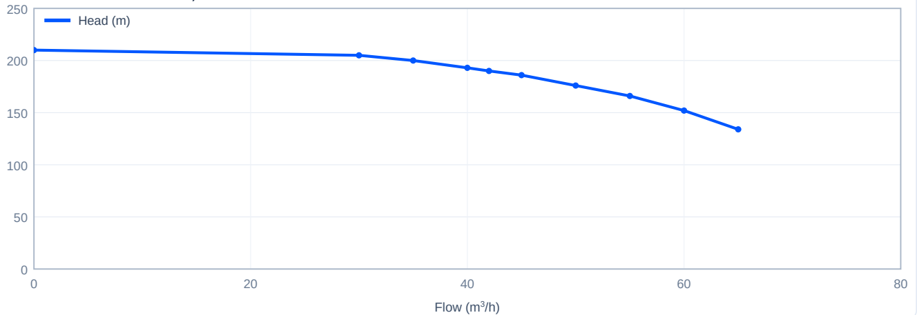
Head versus flow - CDM42-6, 60 Hz
