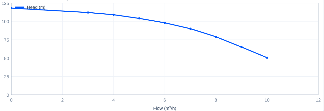
Head versus flow - CDM5-11, 60 Hz
