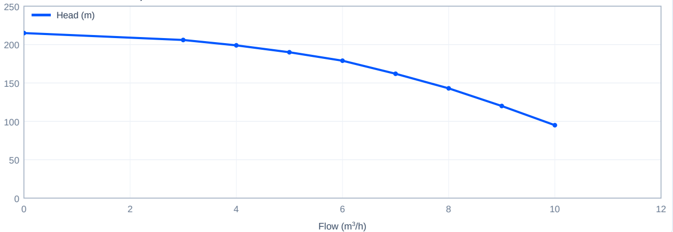
Head versus flow - CDM5-20, 60 Hz
