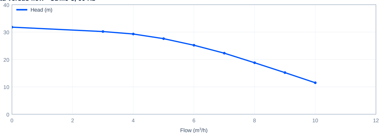
Head versus flow - CDM5-3, 60 Hz
