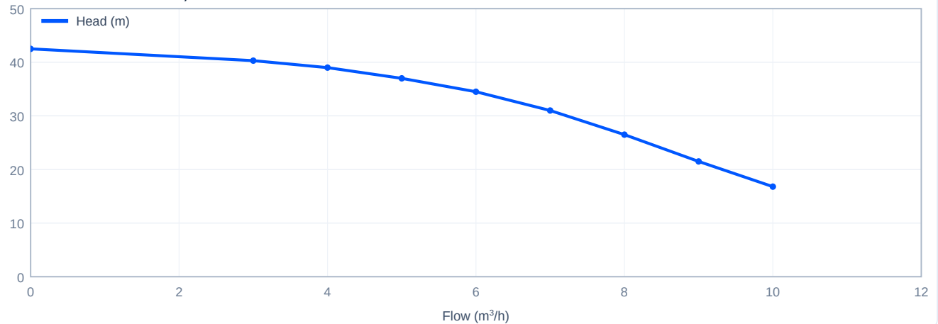
Head versus flow - CDM5-4, 60 Hz
