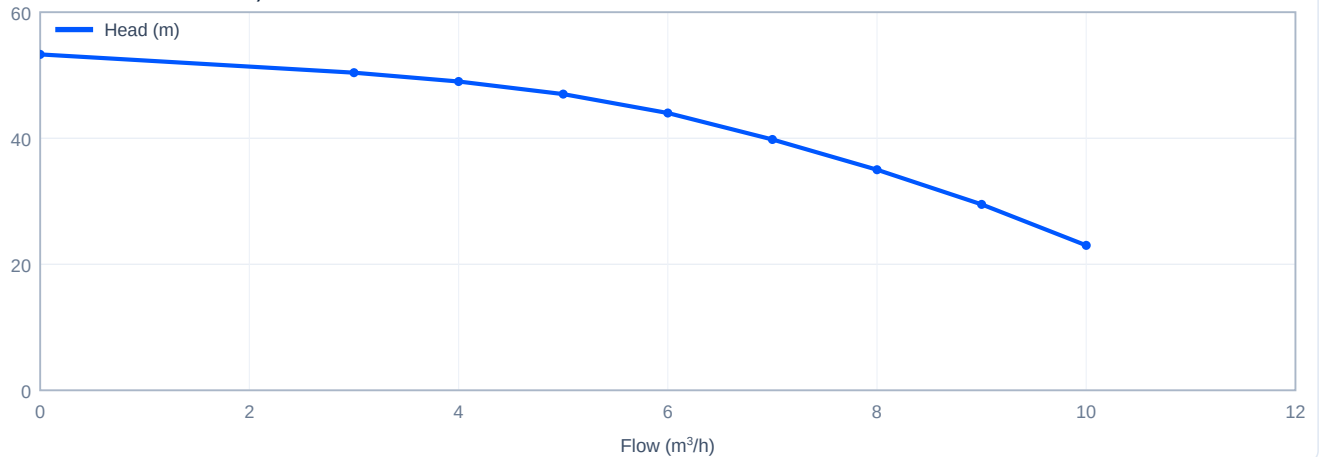
Head versus flow - CDM5-5, 60 Hz
