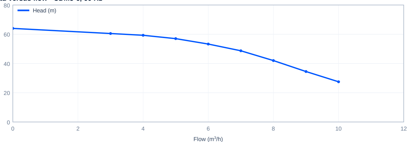
Head versus flow - CDM5-6, 60 Hz
