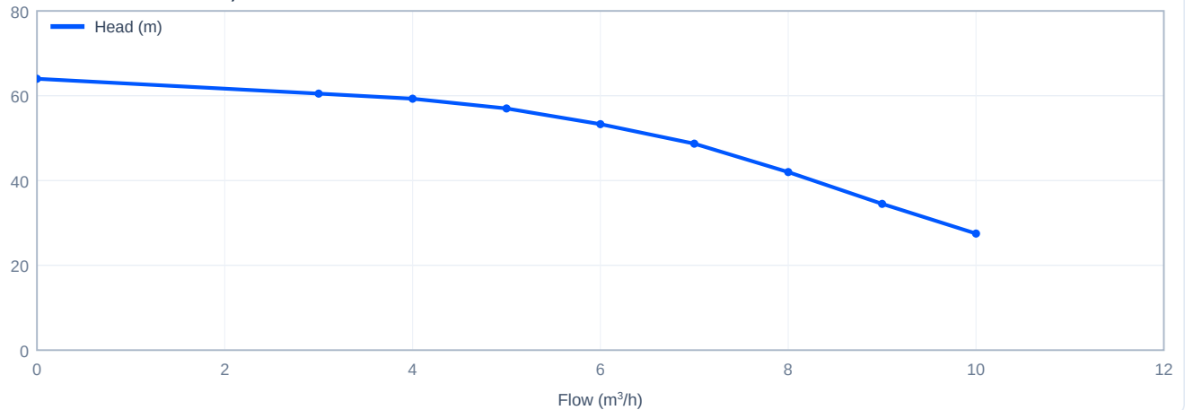
Head versus flow - CDM5-6, 60 Hz
