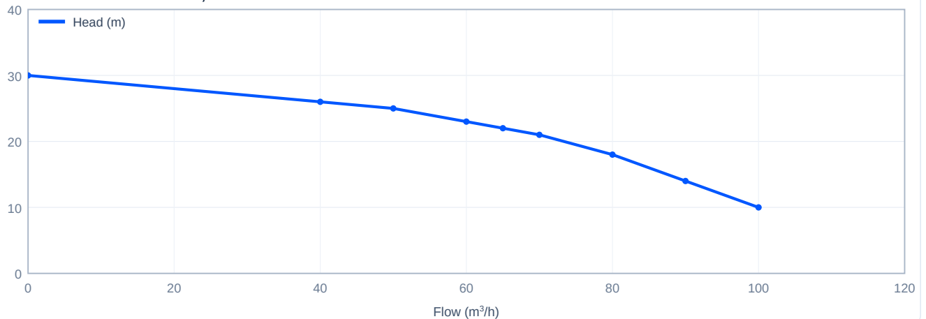
Head versus flow - CDM65-1-1, 60 Hz
