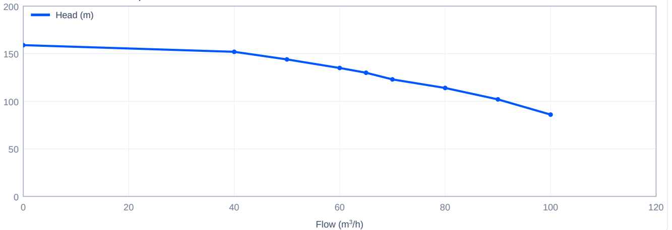
Head versus flow - CDM65-4, 60 Hz
