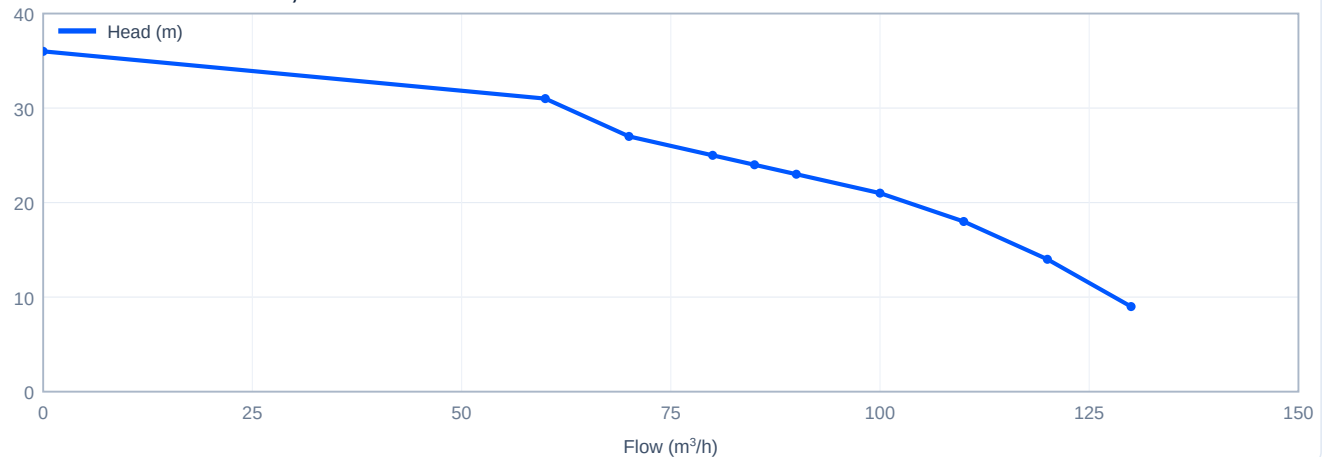
Head versus flow - CDM85-1-1, 60 Hz
