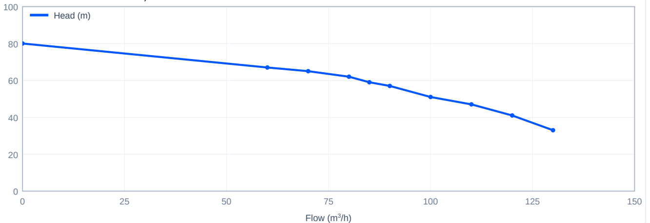
Head versus flow - CDM85-2-1, 60 Hz
