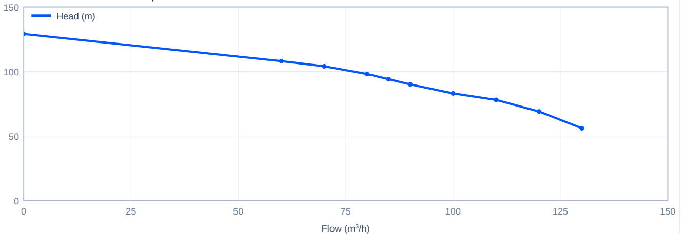
Head versus flow - CDM85-3-1, 60 Hz
